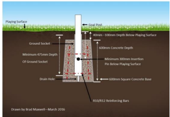
Typical Ground Socket Design
